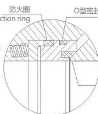
阀座耐火结构 Refractory structure of valve seat
