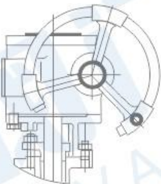
蜗轮传动 Worm gear operation
